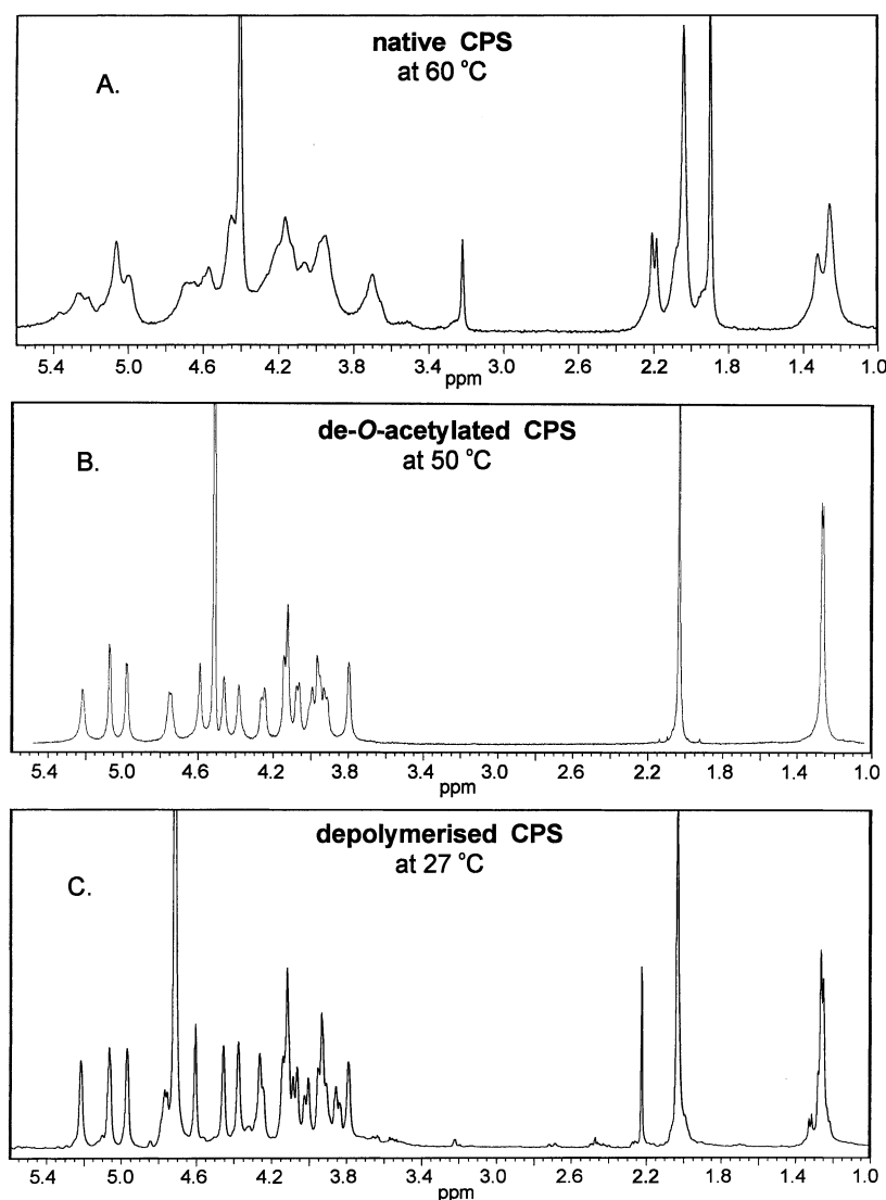
Fig. 1. 1D ^1\text{H} NMR spectra of native S. pneumoniae type 1 CPS (A), O -deacetylated CPS (B) and CPS after periodate oxidation and base degradation (C). The resonance at 2.225 ppm in C is acetone as internal standard.
