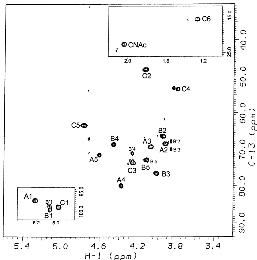
Fig. 3. 500-MHz ^{13}\text{C} -decoupled HMQC spectrum of the depolymerized S. pneumoniae type 1 CPS ( Spt1 ) at 27 °C. The letters refer to the residues in Fig. 2. The A H-1– A C-1 cross peak is labeled A1, etc. The anomeric and methyl regions are inserts in the lower left and upper right corner, respectively.
